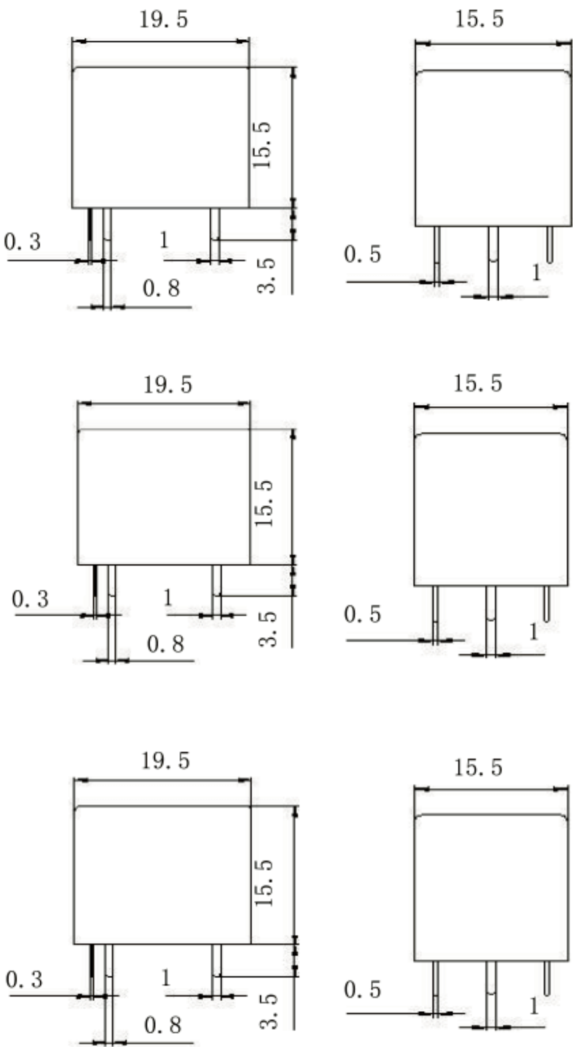
Outline Dimensions
