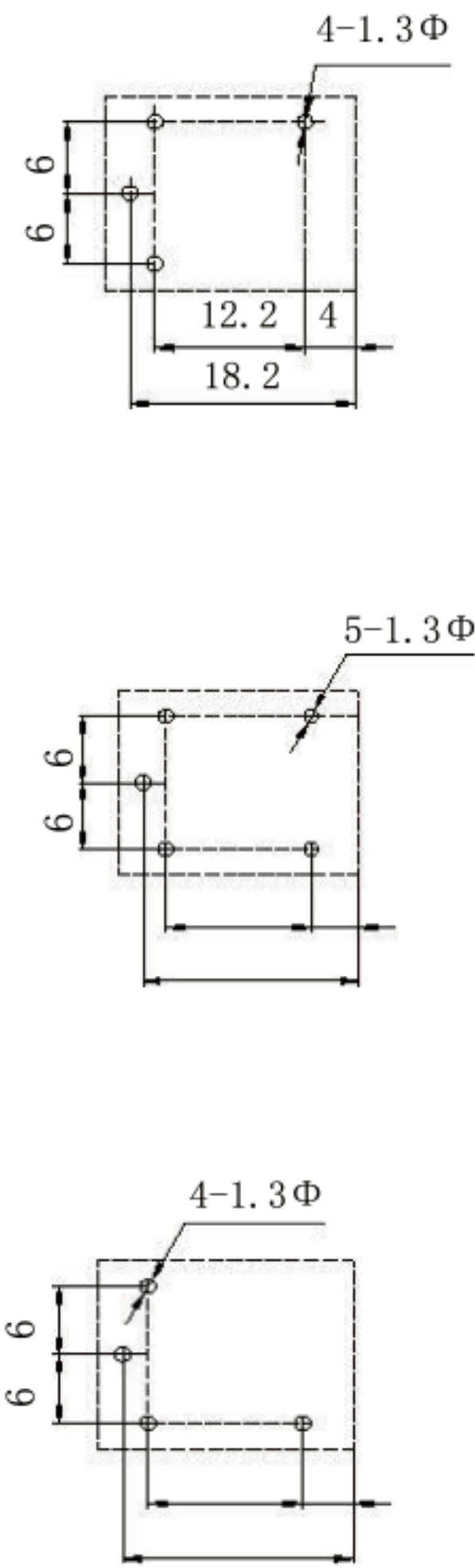
PCB Layout (Bottom view)
